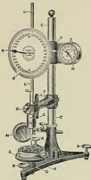
FIG. 163.—Penetrometer.
